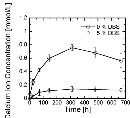
Figure 8. Calcium ion concentration profile.
